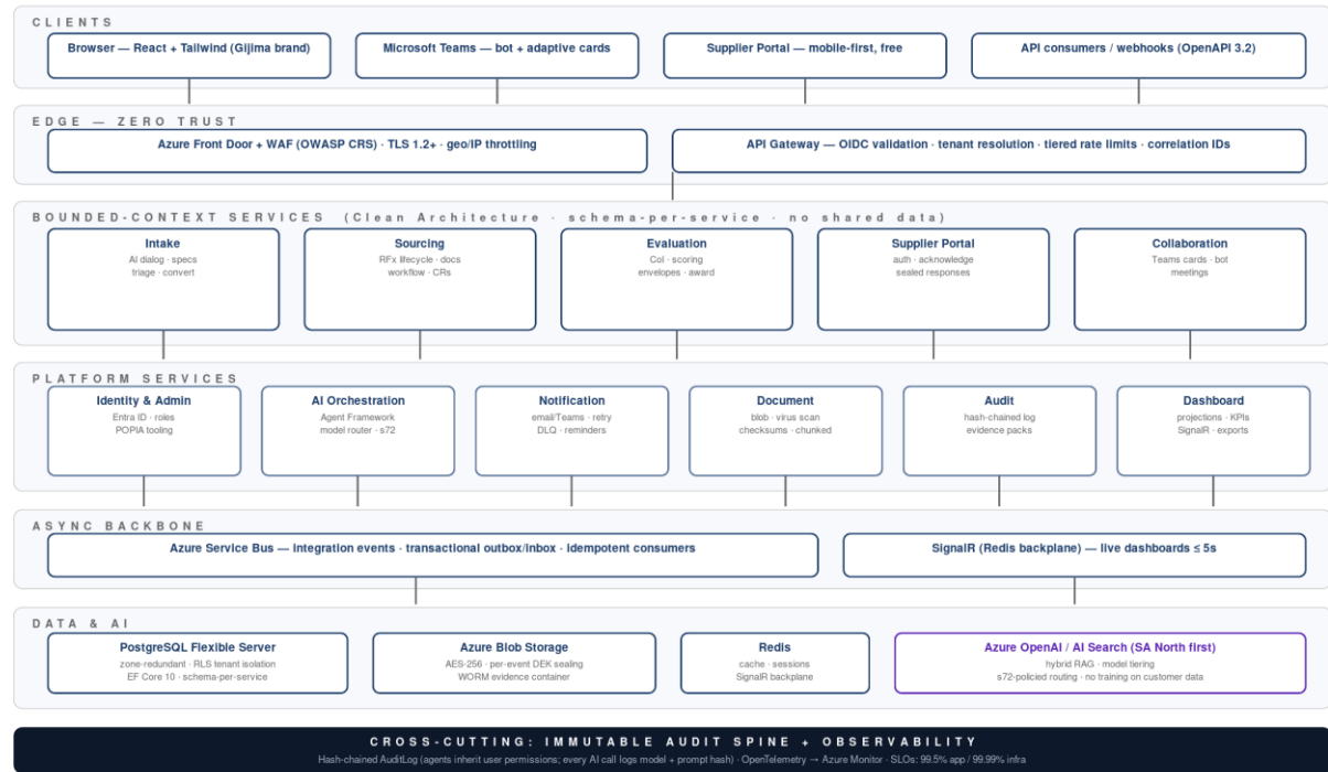
Figure 6 — System architecture: services, async backbone, data & AI, audit spine
